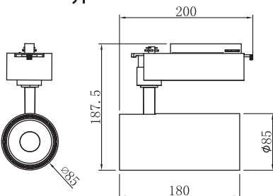
35W type
